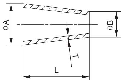
Concentric reducer D.L31
