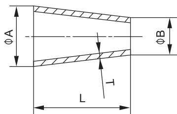
Concentric reducer S.L31
