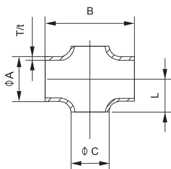
Reducing short cross S.9WWWW
