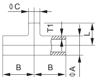
Reducing short tee D.7W
