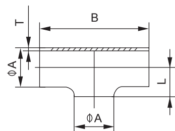
Pull tee
