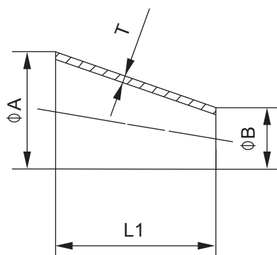
Eccentric reducer D.L32
