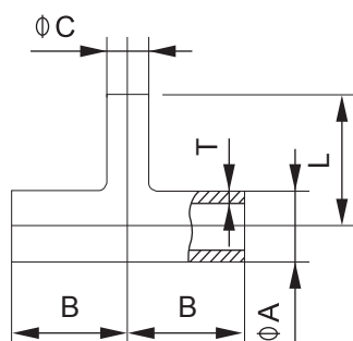
Reducing tee D.L7W
