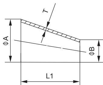
Eccentric reducer S.L32
