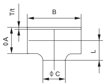
Reducing short tee S.7RW
